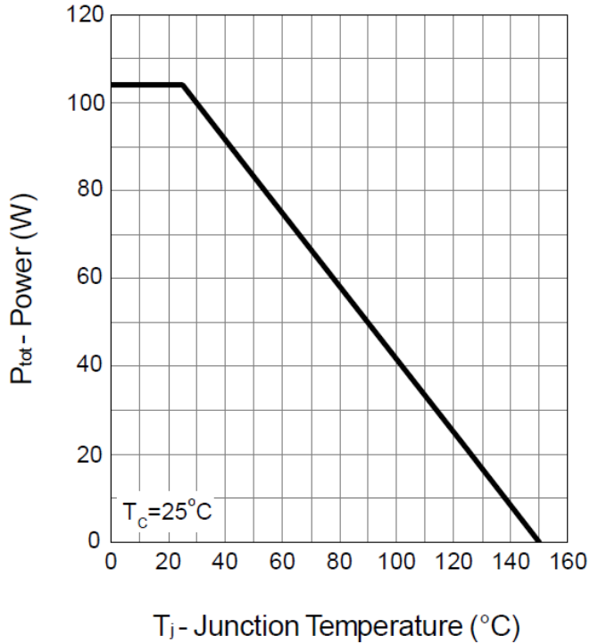
Power Dissipation
