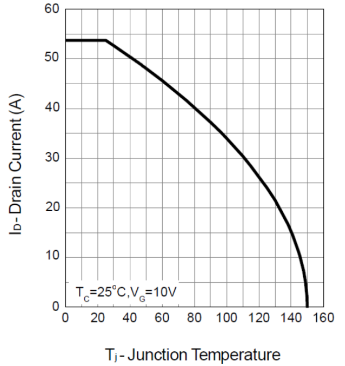
Drain Current
