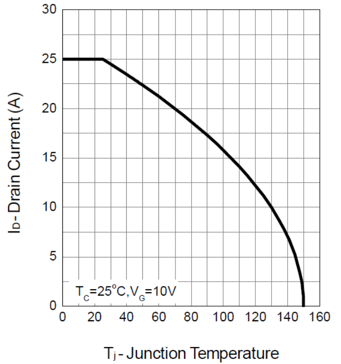
Drain Current
