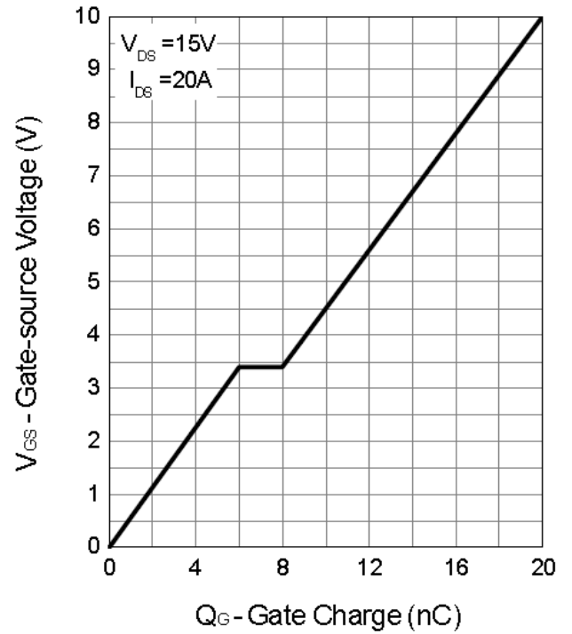
Gate Charge
