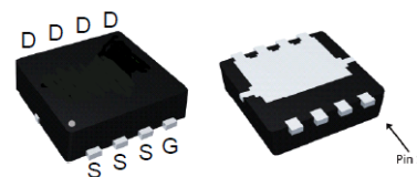
DFN3.3x3.3-8
